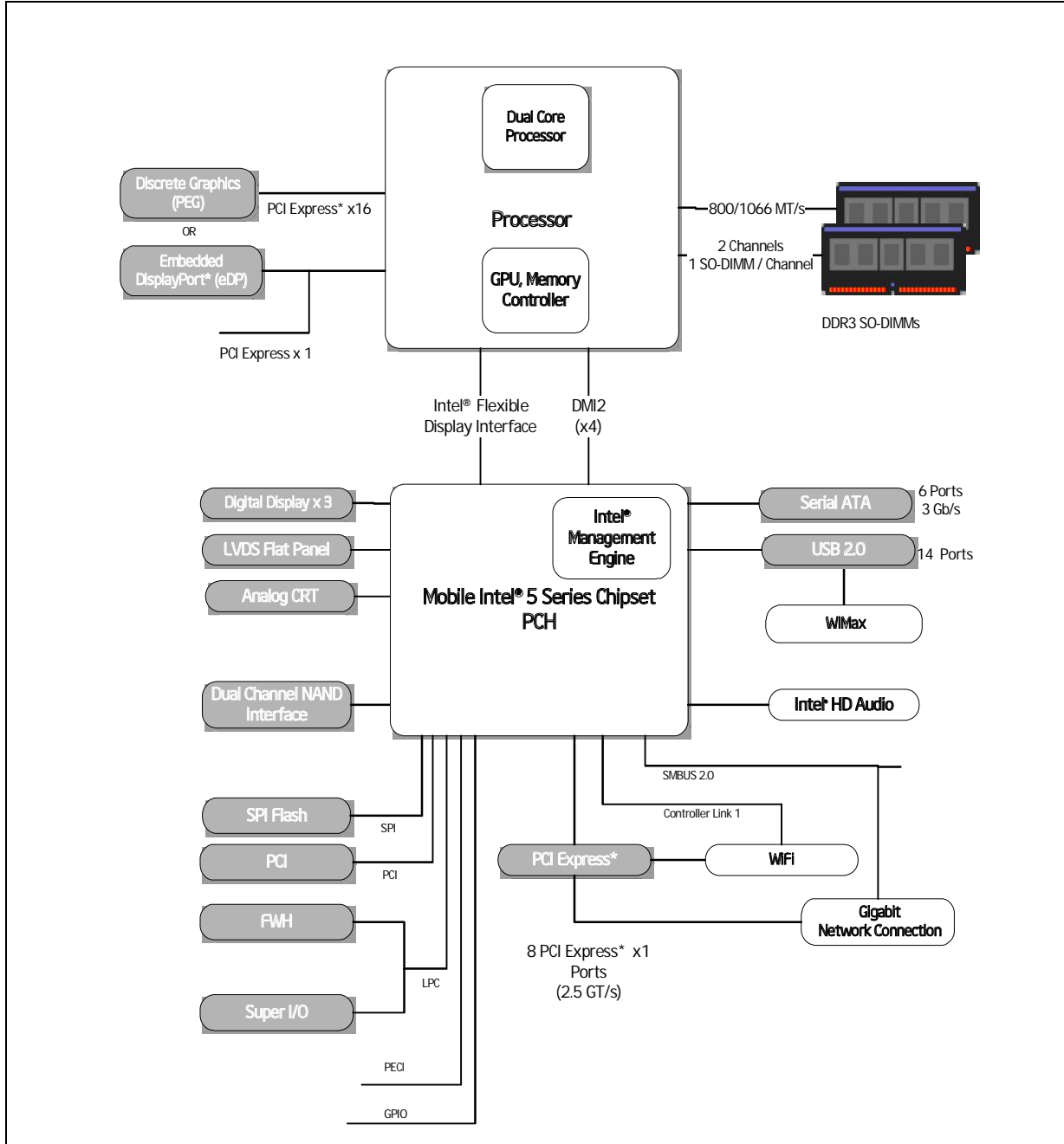
Figure 1-1. Intel® Pentium® P6000 and U5000 Mobile Processor Series on the Calpella Platform
