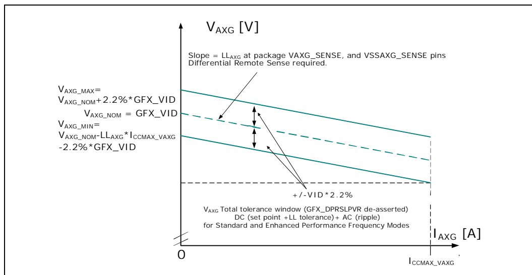
Figure 7-15. V_{AXG}/I_{AXG} Static and Ripple Voltage Regulation
